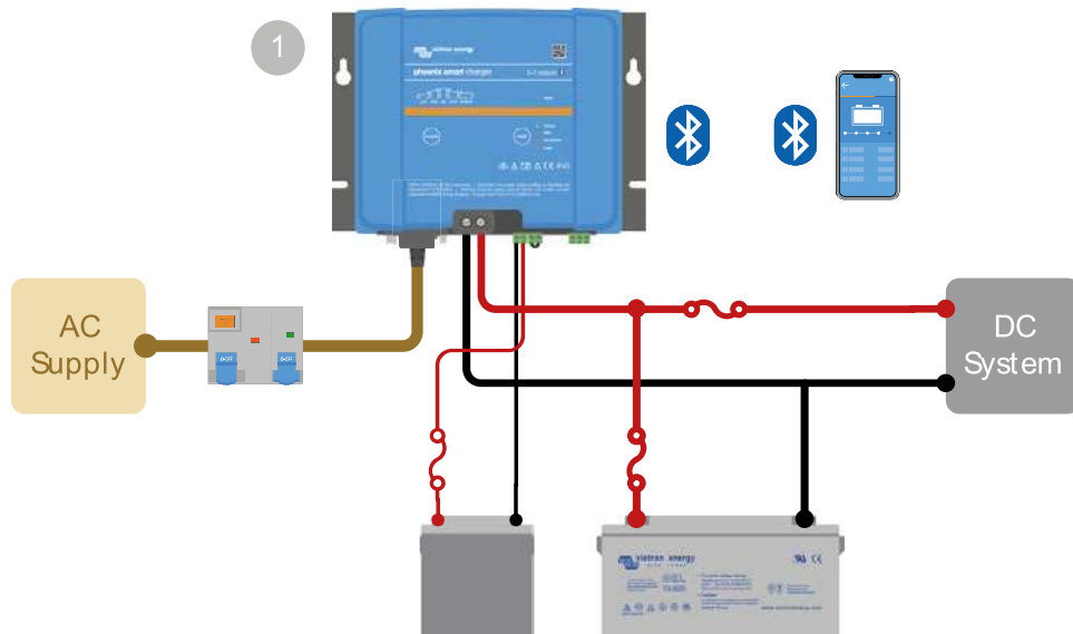
Battery charger used to charge a main battery and provides a maintenance charge to a smaller battery, like a generator starter battery.
